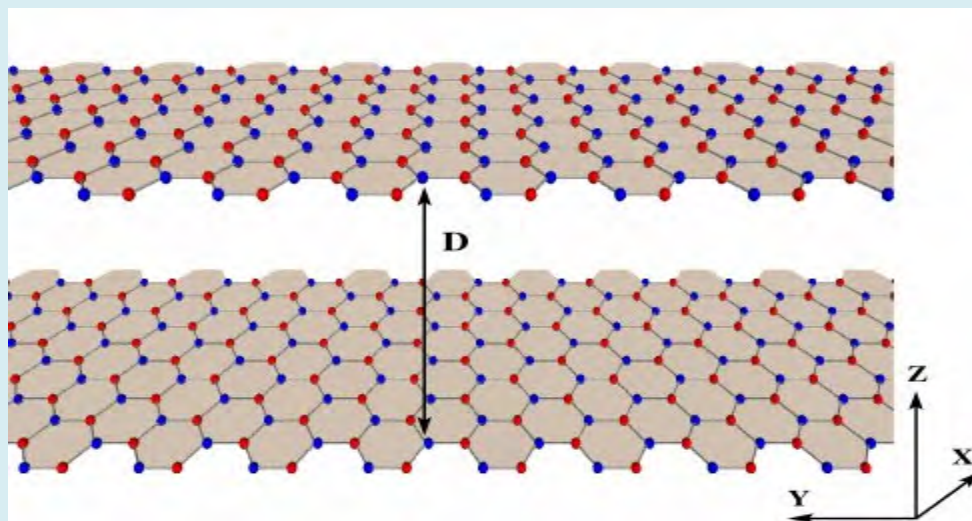
Figure 1: Color online- Schematic depicting 2 un-doped and un-strained freely suspended graphene layers separated by a finite distance ( D ) [1].
